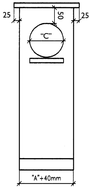
Front Elevation
