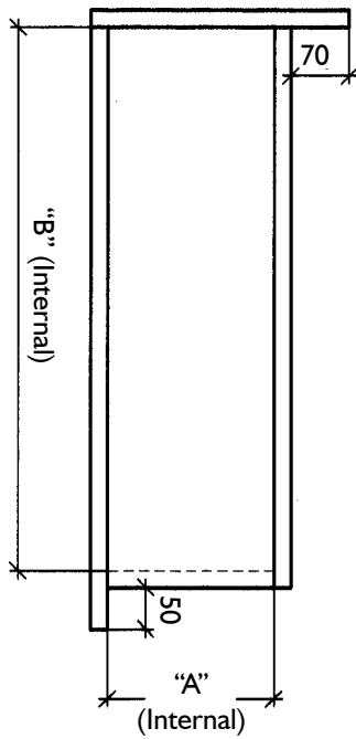
Side Elevation
